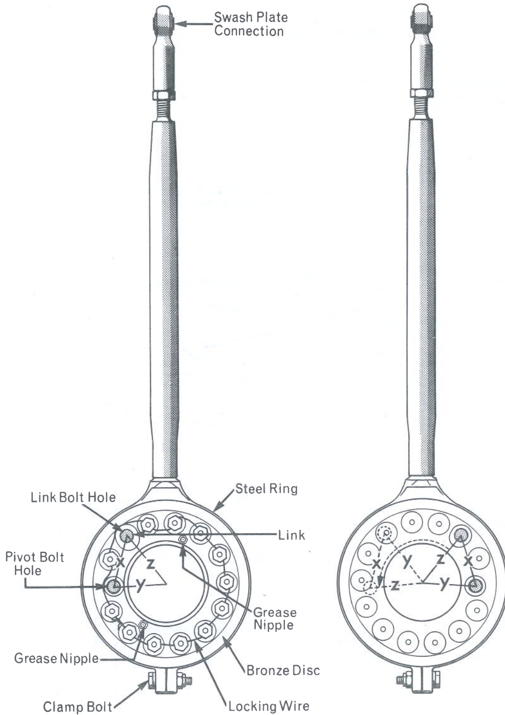
FRONT VIEW (CORRECT)
