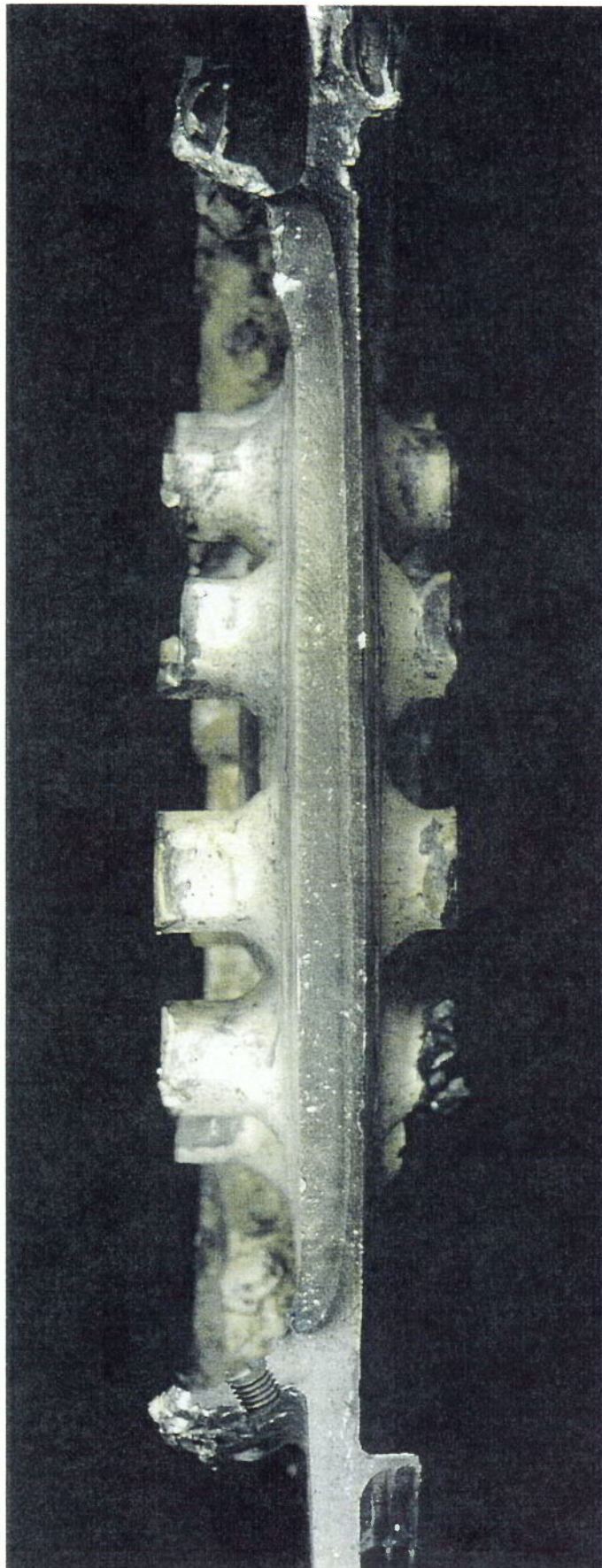
G-OJEM'S NO 2 ENGINE HP TURBINE DISC FRACTURE SURFACE
