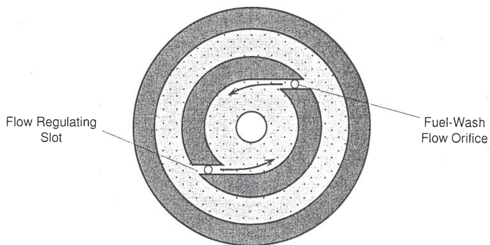
SWIRL CHAMBER
