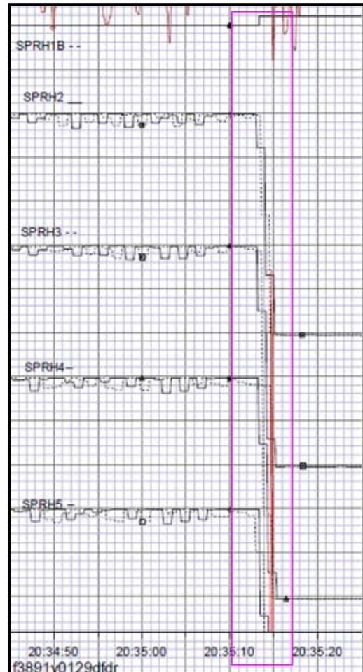
Pic. 16 – Spoilers extension graphic
