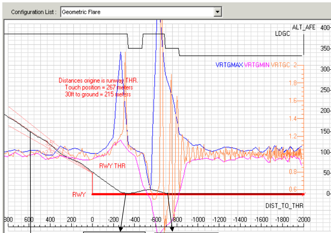
Pic. 14 – Both touchdown main landing gears graphic.
