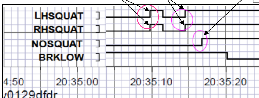
Pic. 15 – Main and nose gears' sensors graphic.
